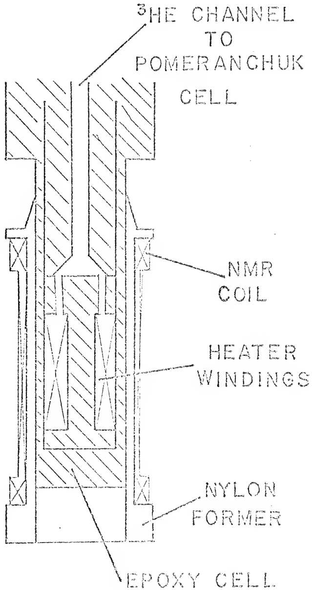
Fig. 7 NMR region of Susceptibility Cell.
